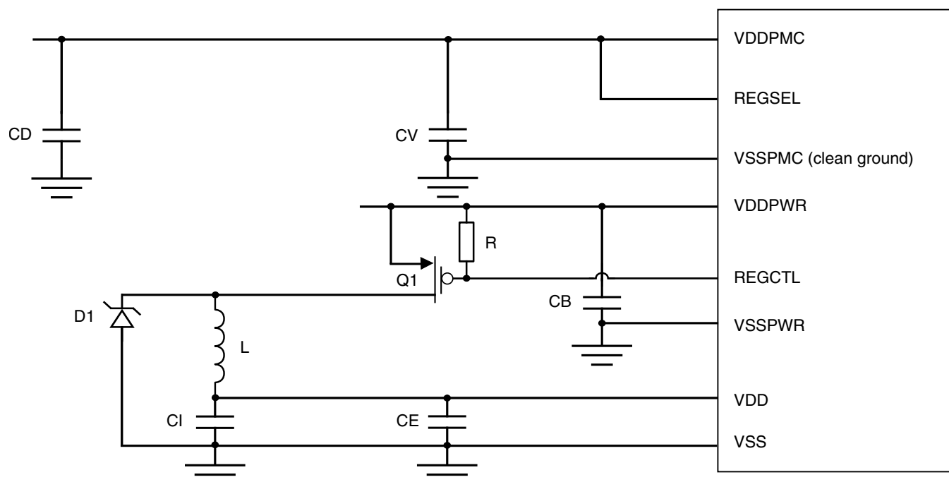
Figure 12. SMPS configuration
