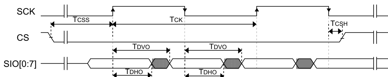
Figure 43. FlexSPI output timing in DDR mode
