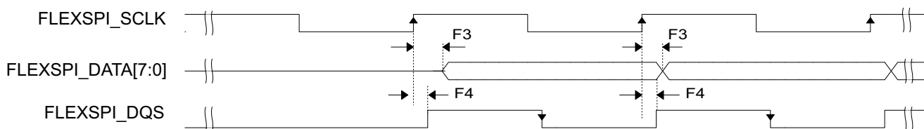
Figure 38. FlexSPI input timing in SDR mode where FlexSPIn_MCR0[RXCLKSRC] = 0x3 (Case A1)
