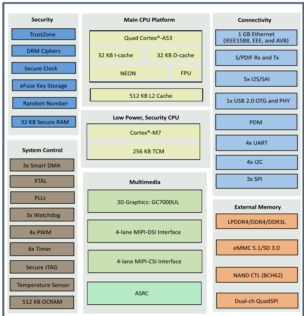
Figure 1. i.MX 8M Nano system block diagram
