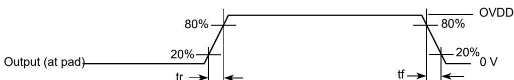
Figure 9. Output transition time waveform
