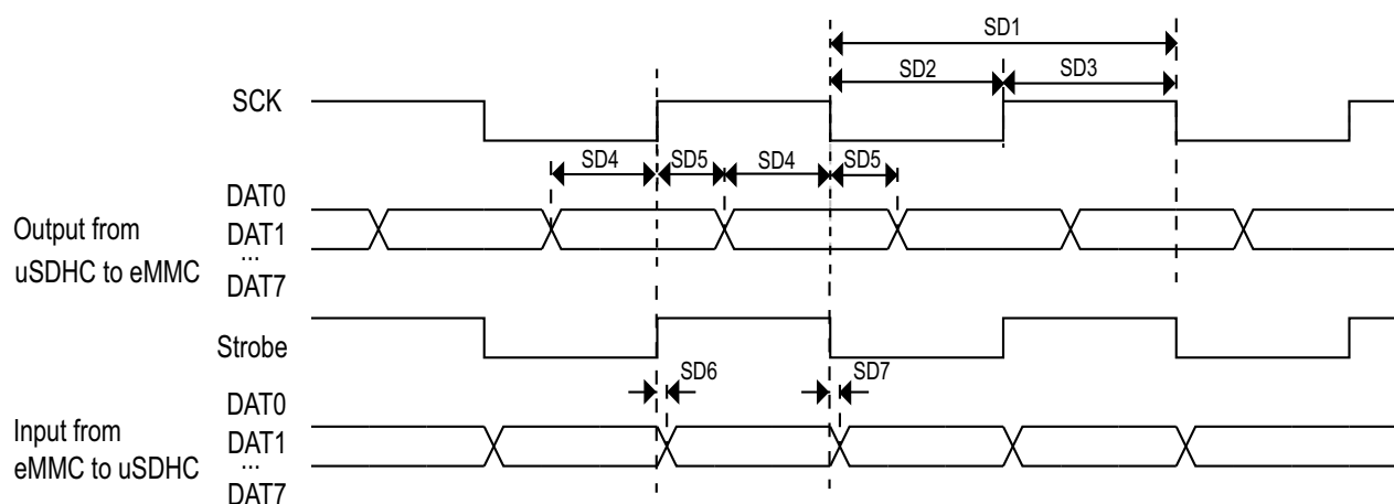
Figure 17. HS400 Mode timing
