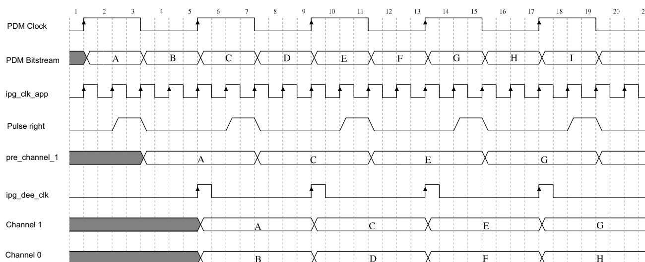
Figure 35. PDM input timing
