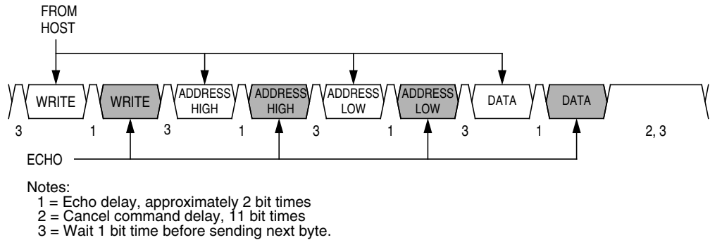
Figure 18-15. Write Transaction
