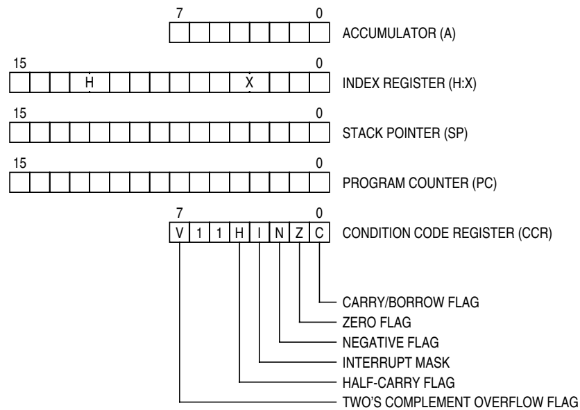
Figure 8-1. CPU Registers
