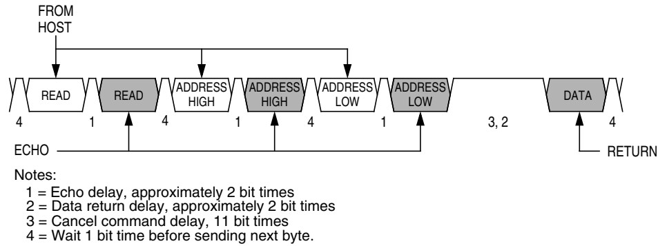
Figure 18-14. Read Transaction
