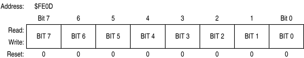
Figure 16-5. Break Address Register (BRKL)
