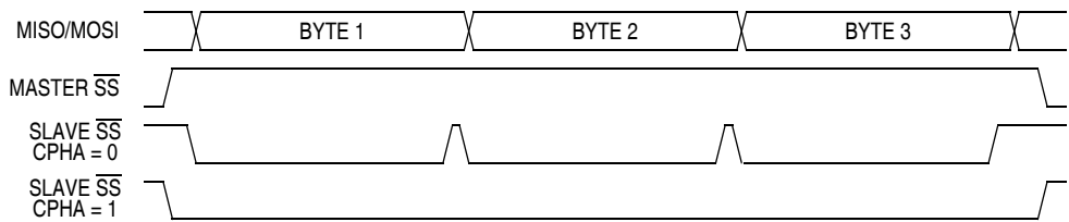
Figure 14-13. CPHA/SS Timing
