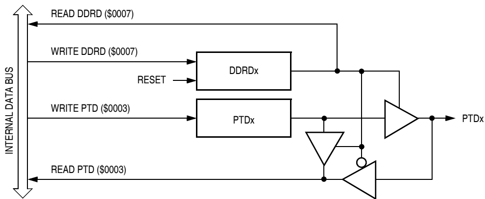
Figure 11-13. Port D I/O Circuit
