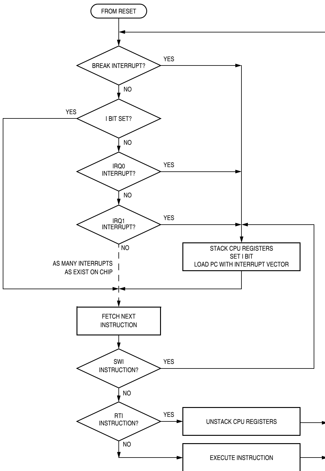
Figure 13-11. Interrupt Processing
