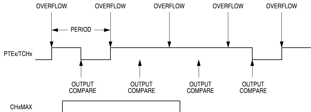
Figure 15-9. CHxMAX Latency
