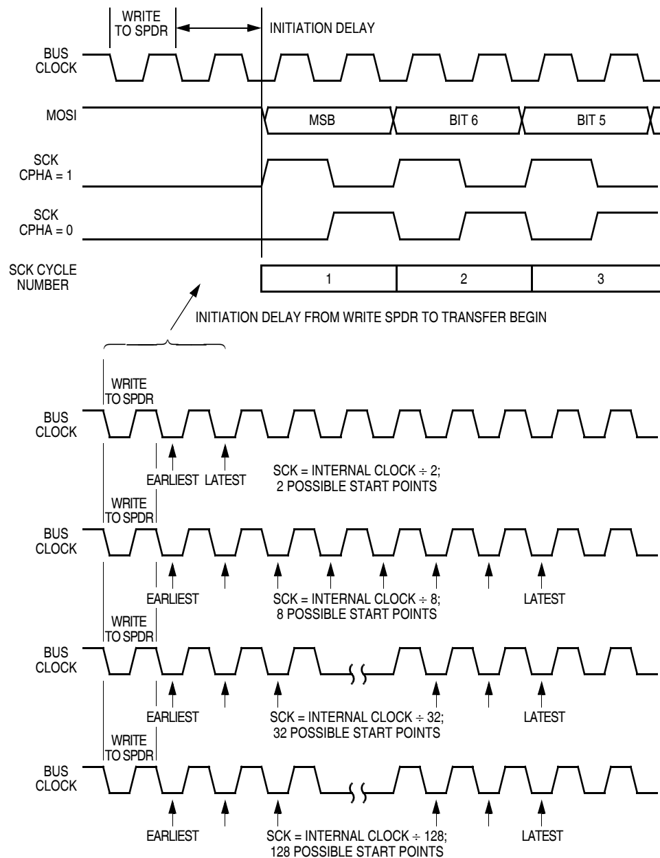
Figure 14-8. Transmission Start Delay (Master)
