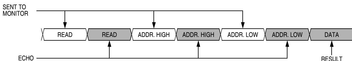
Figure 16-9. Read Transaction
