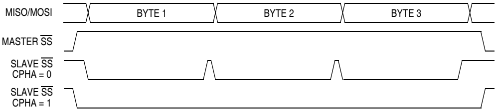
Figure 14-6. CPHA/\overline{SS} Timing
