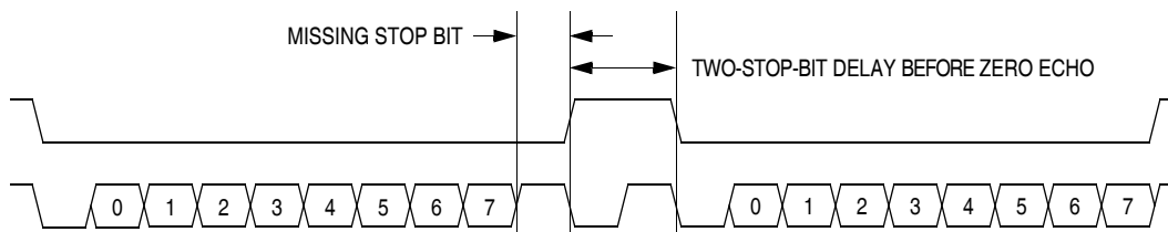
Figure 16-10. Break Transaction
