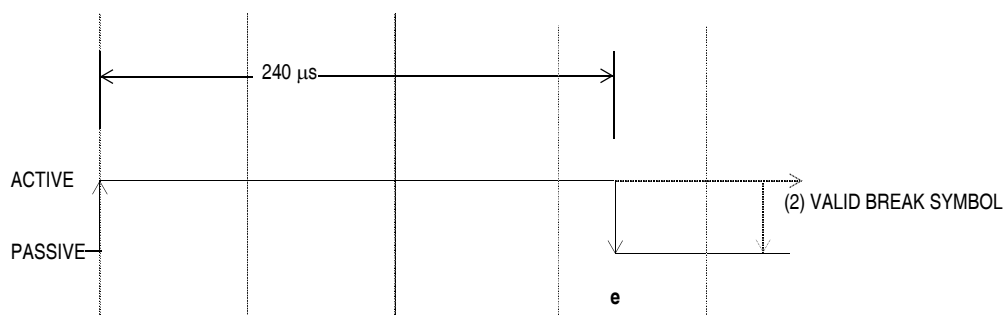
Figure 4-12. J1850 VPW Received BREAK Symbol Times
