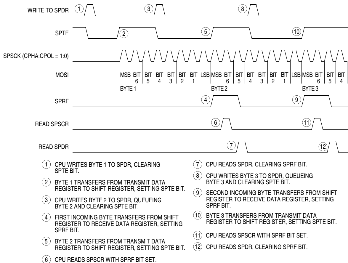
Figure 14-12. SPDR/SPTE CPU Interrupt Timing
