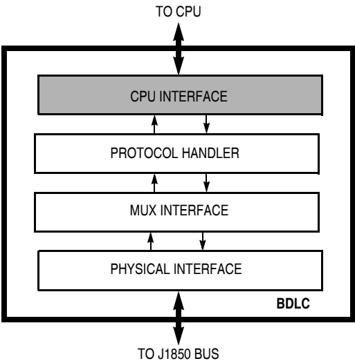
Figure 4-16. BDLC Block Diagram
