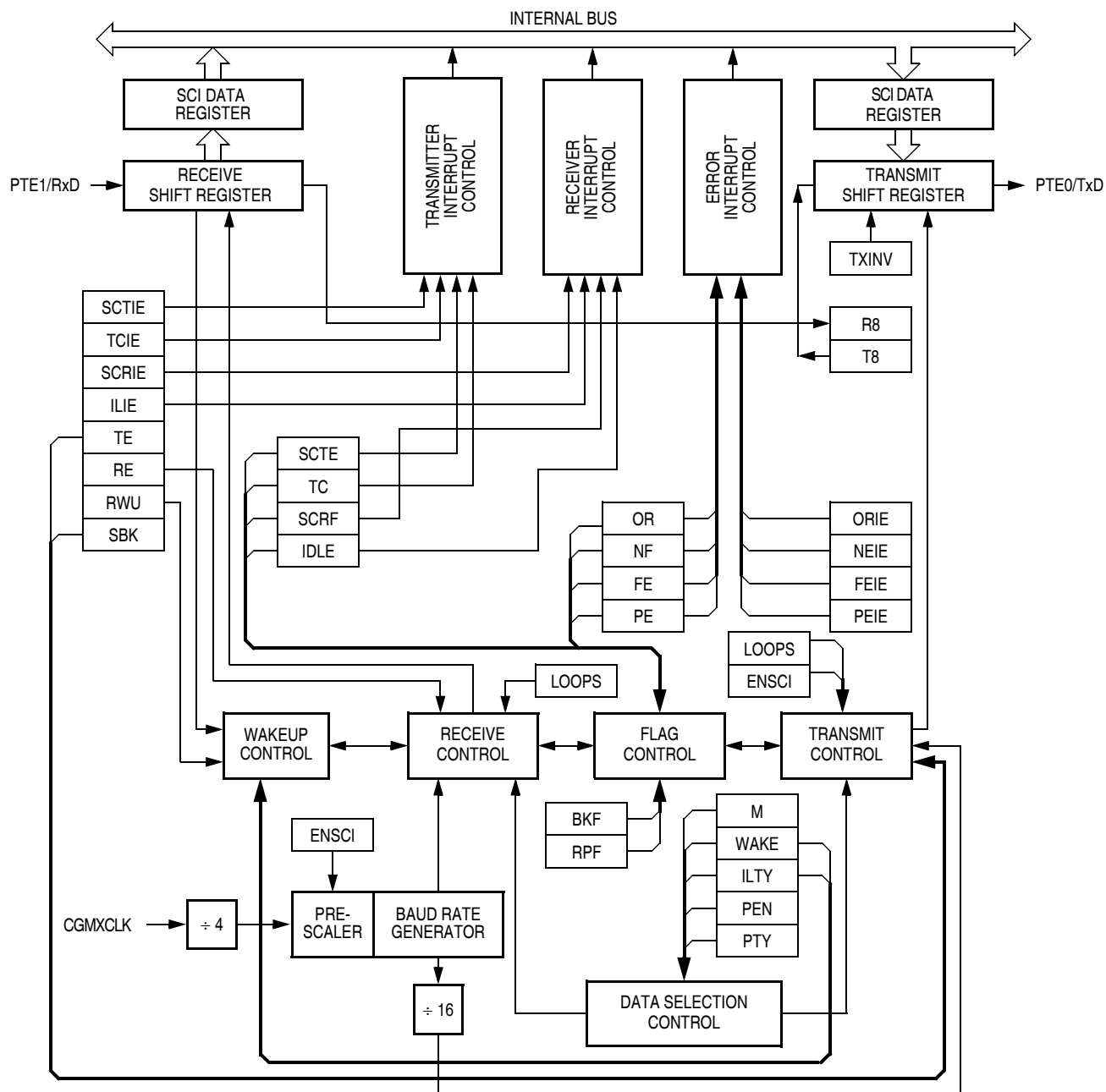
Figure 12-3. SCI Module Block Diagram
