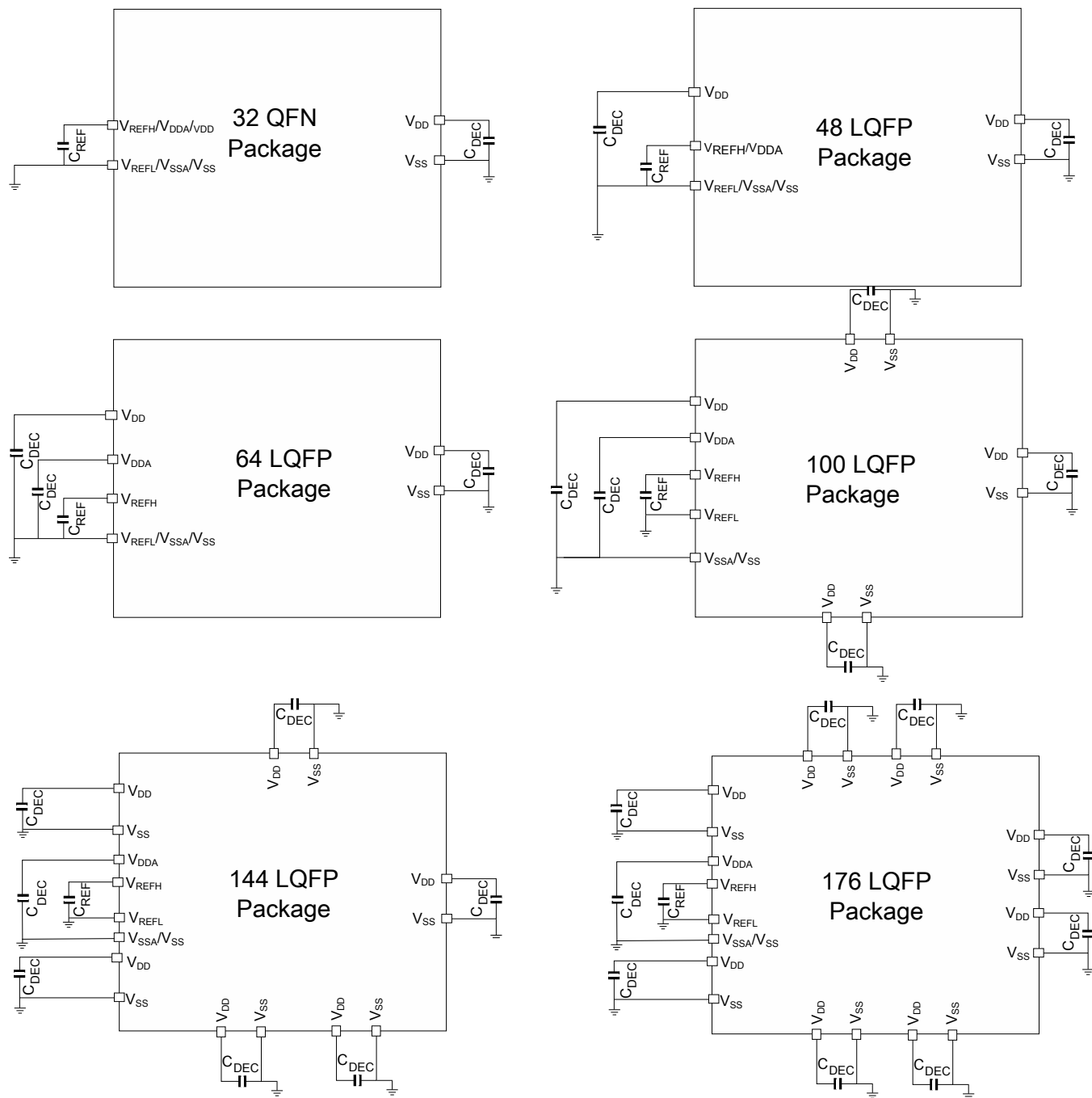
Figure 6. Pinout decoupling
