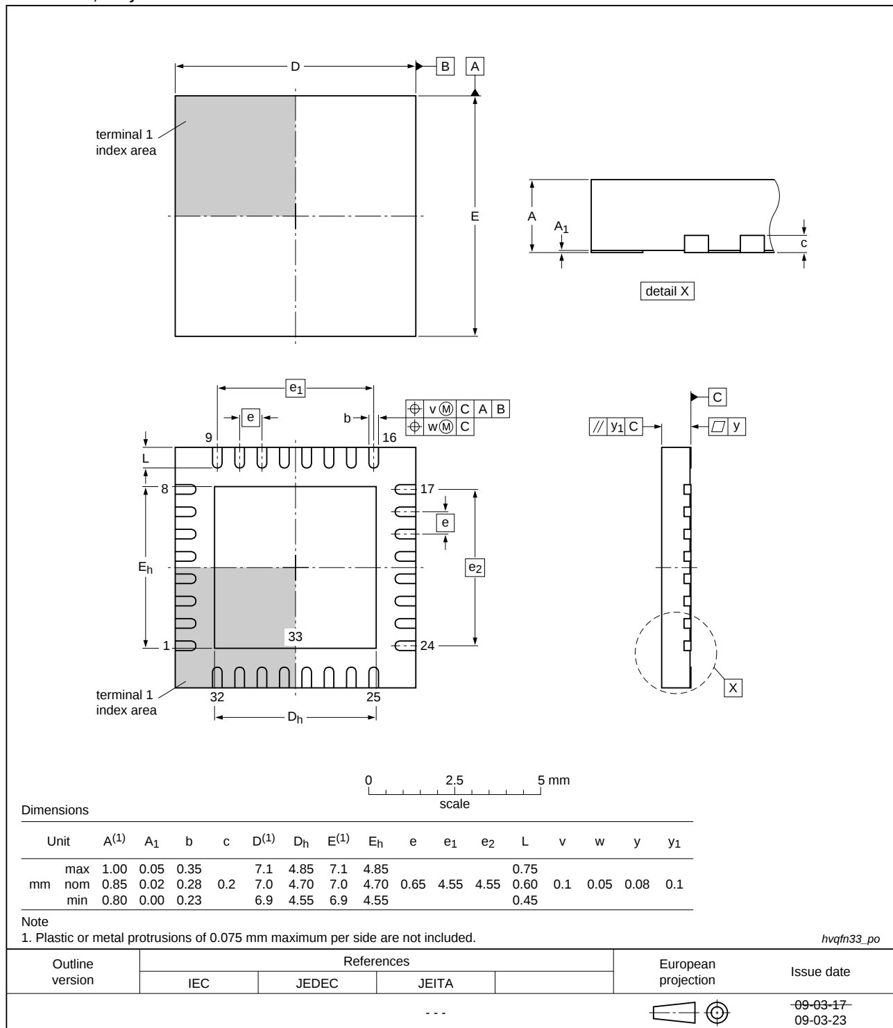
Fig 35. Package outline HVQFN33 (7 x 7 x 0.85 mm)
