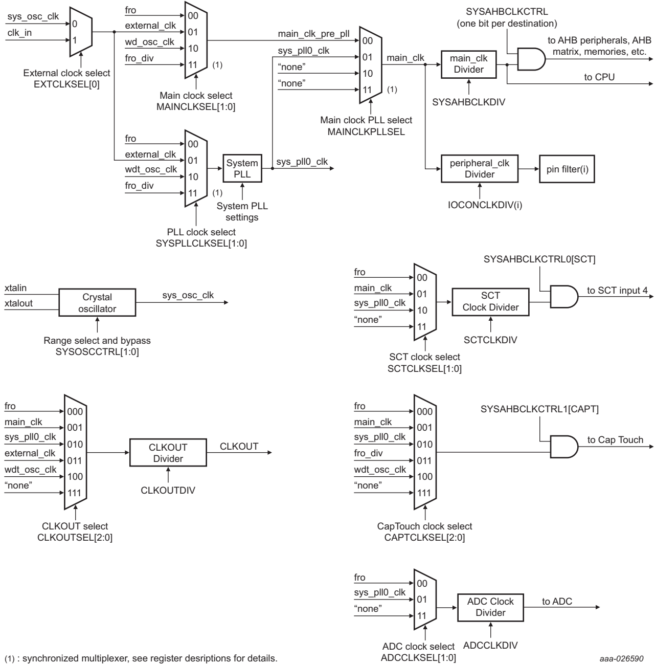
Fig 11. LPC84x clock generation
