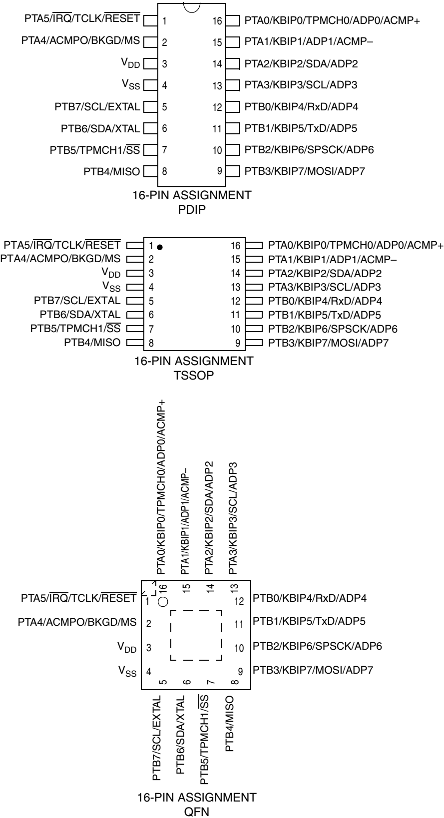
Figure 2-2. 16-Pin Packages
