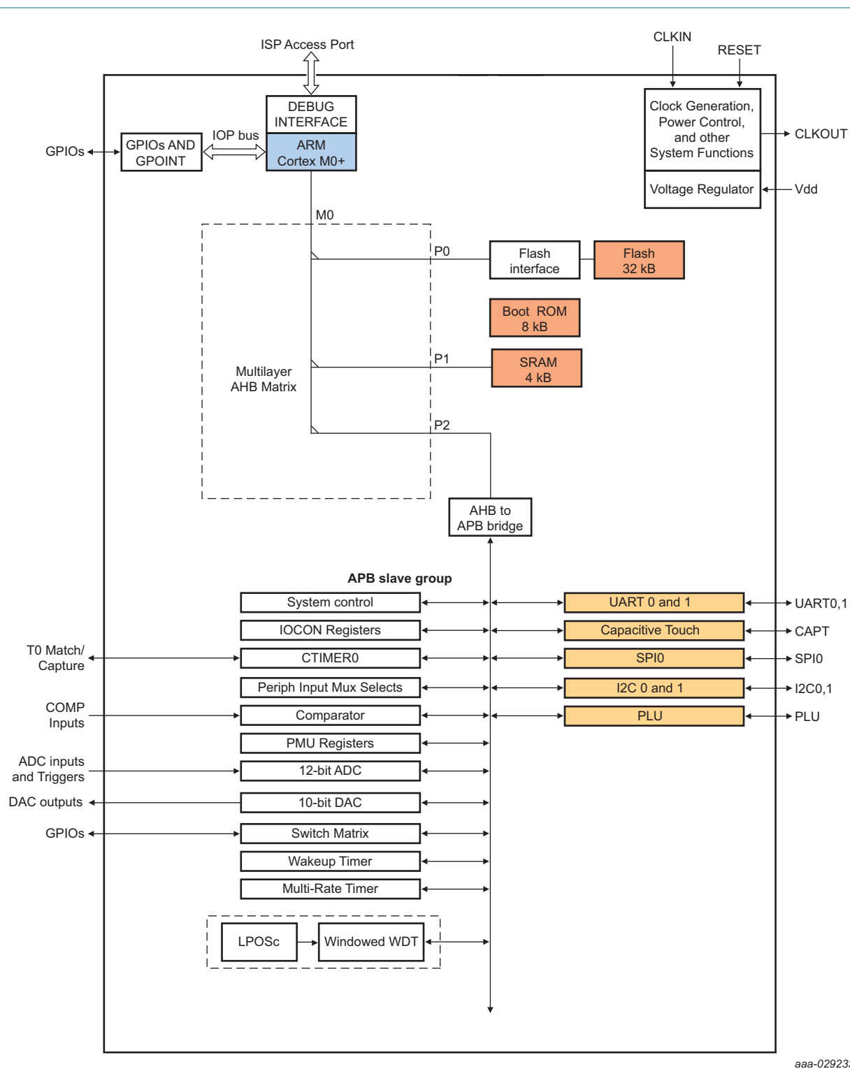
Fig 4. LPC804 block diagram
