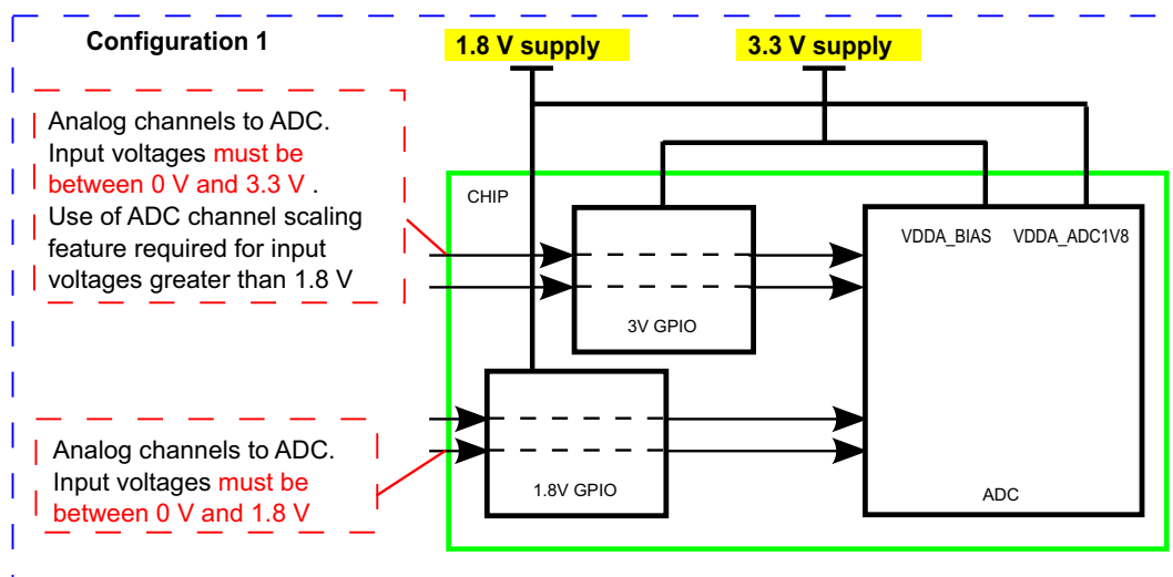
Fig 39. Configuration 1
