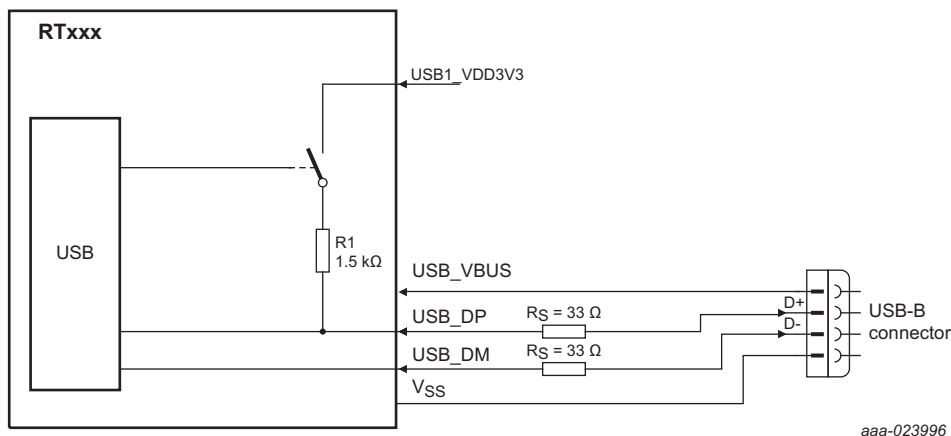
Fig 37. USB interface on a self-powered device where USB_VBUS = 5 V
