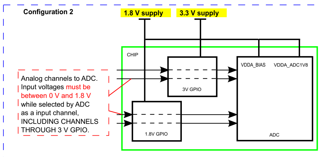
Fig 40. Configuration 2
