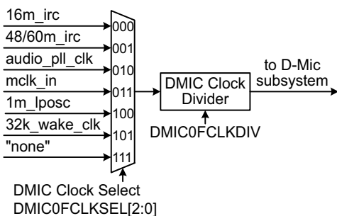
Fig 8. RT600 clock generation (continued)
