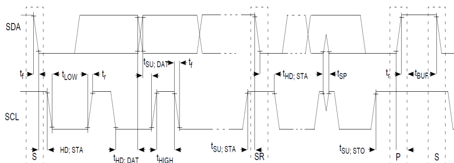
Fig 27. Timing definition for devices on the I2C bus
