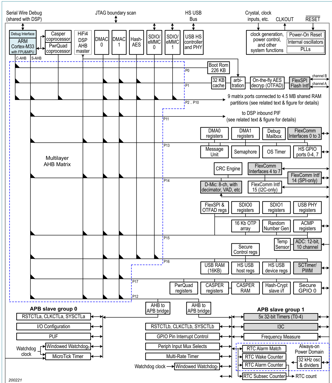
Fig 4. Block diagram - Cortex-M33 view (Not all features are available in all packages. Flexcomm Interfaces 0 through7 each include USART, SPI, I2C, and I2S functions. Grey-shaded blocks indicate peripherals that provide DMA requests or are otherwise able to trigger DMA transfers. Hash-AES and SDIO include a dedicated DMA function.)
