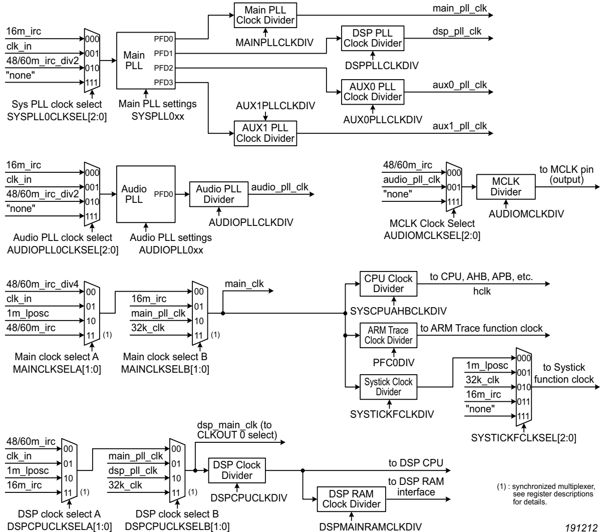
Fig 6. RT600 clock generation
