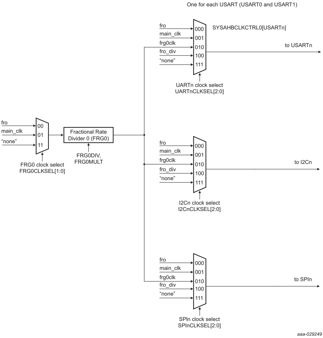
Fig 13. LPC804 clock generation (continued)
