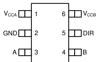
图 5-2. DCK Package 6-Pin SC70 Top View
