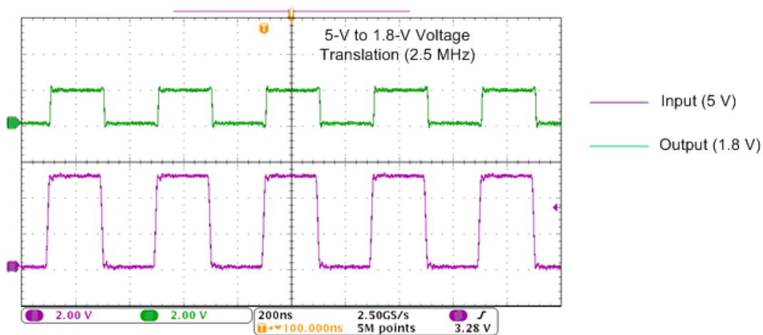
图 8-4. Translation Down (5 V to 1.8 V) at 2.5 MHz
