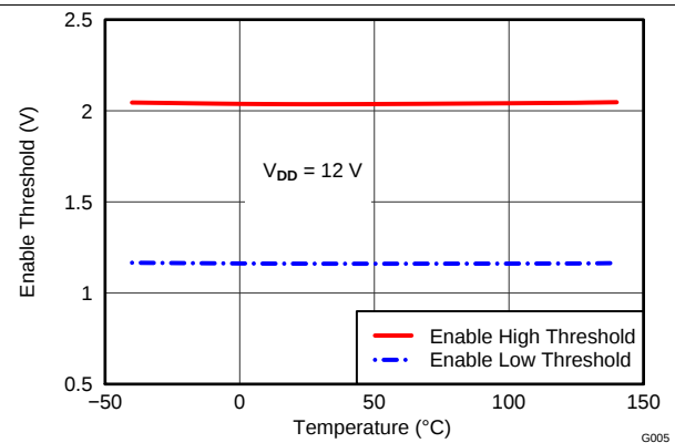
图 8. Enable Threshold vs Temperature
