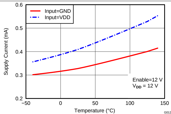
图 5. Supply Current vs Temperature (Outputs In DC On/Off Condition)
