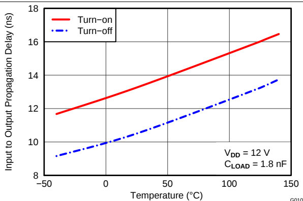
图 13. Input to Output Propagation Delay vs Temperature
