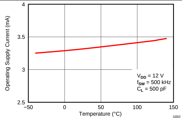
图 4. Operating Supply Current vs Temperature (Outputs Switching)
