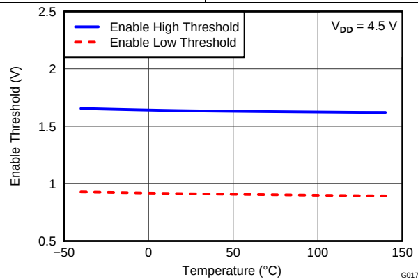
图 19. Enable Threshold vs Temperature
