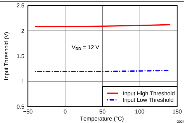
图 7. Input Threshold vs Temperature
