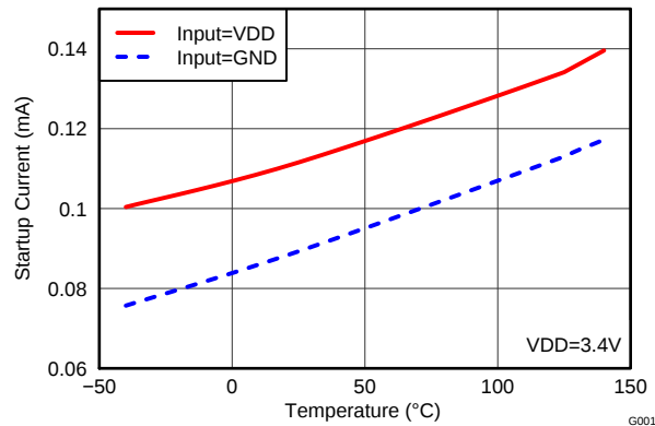
图 3. Start-Up Current vs Temperature
