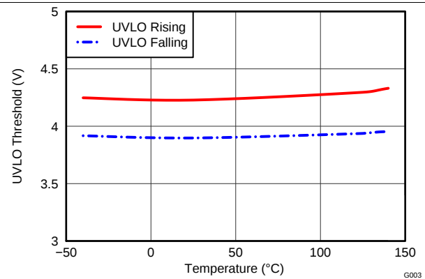
图 6. UVLO Threshold vs Temperature
