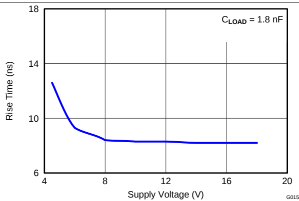
图 17. Rise Time vs Supply Voltage
