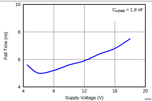
图 18. Fall Time vs Supply Voltage
