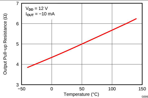
图 9. Output Pullup Resistance vs Temperature
