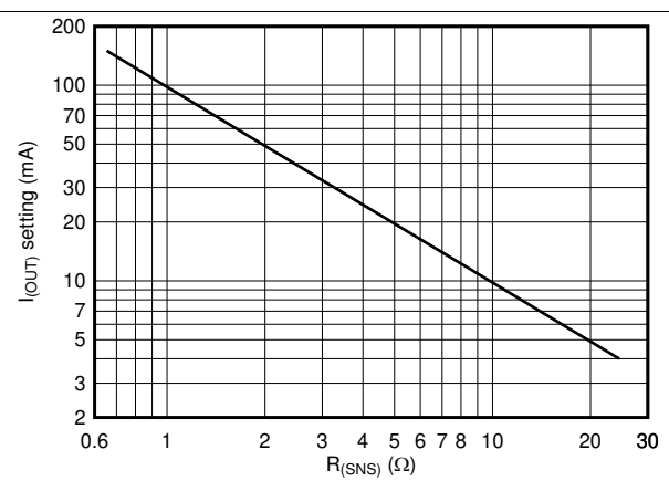
图 3. Output Current vs Current-Sense Resistor
