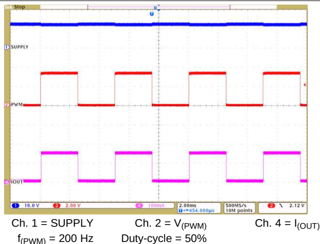
图 8. PWM Dimming at 200 Hz
