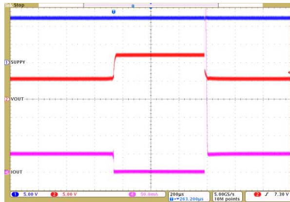
图 10. LED Open-Circuit and Recovery
