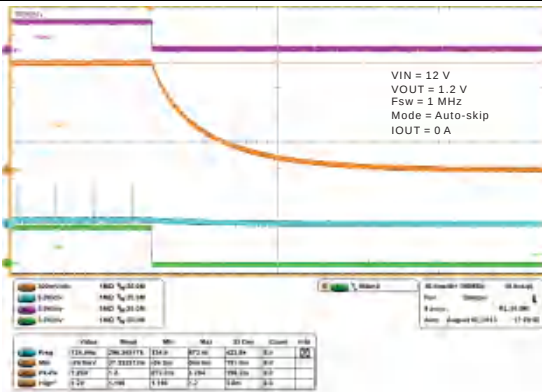
图 25. Shutdown Operation
