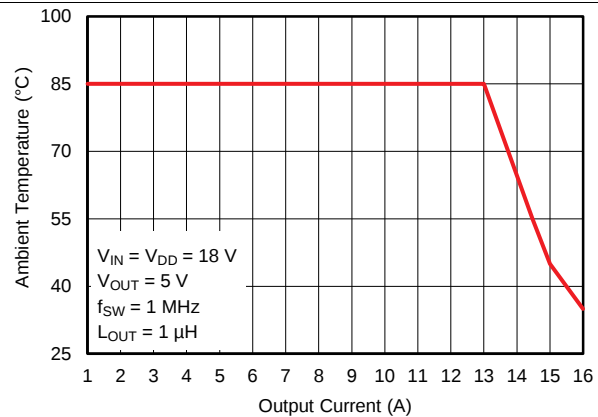
图 12. Safe Operating Area, V_{OUT} = 5\text{ V}
