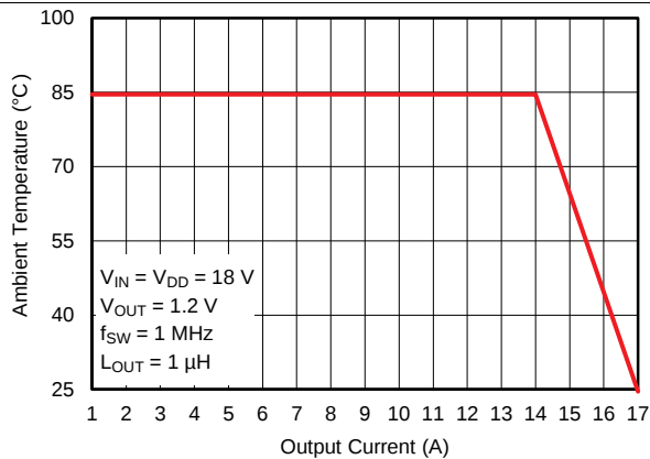
图 11. Safe Operating Area, V_{OUT} = 1.2\text{ V}
