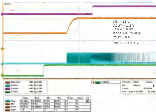
图 29. Pre-Bias Operation
