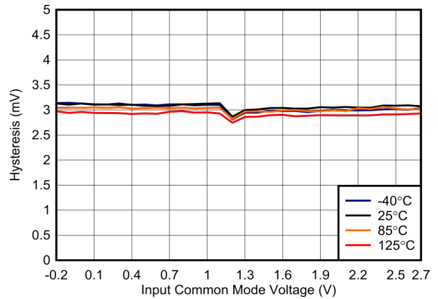
图 6-6. TLV3601 Hysteresis vs. Common-Mode, 2.5 V
