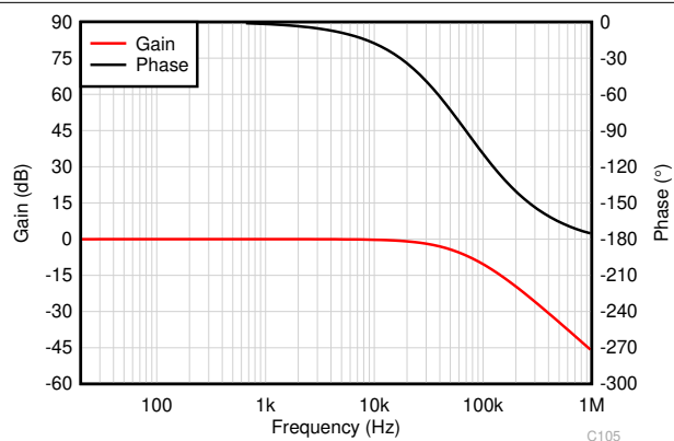
图 9-6. Gain and Phase Response for Current-to-Voltage Buffer
