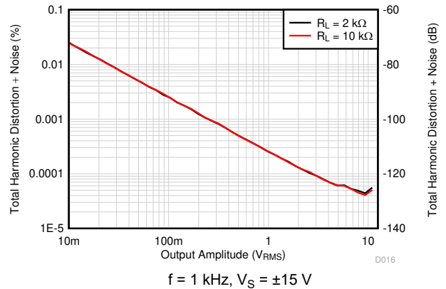
图 6-4. Total Harmonic Noise + Distortion vs Amplitude
