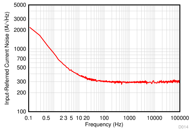
图 6-2. Current Noise vs Frequency
