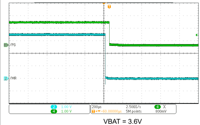
图 10-13. \overline{\text{PG}} \overline{\text{MR}} Level Shift Function - \overline{\text{MR}} Falling
