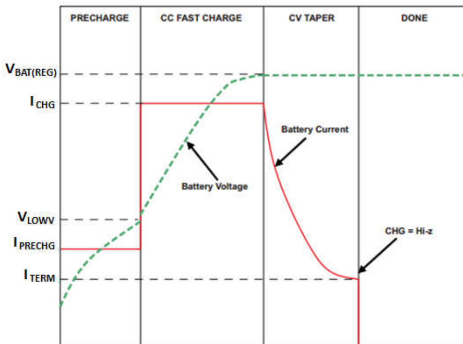
图 9-2. BQ25155 Typical Charge Cycle
