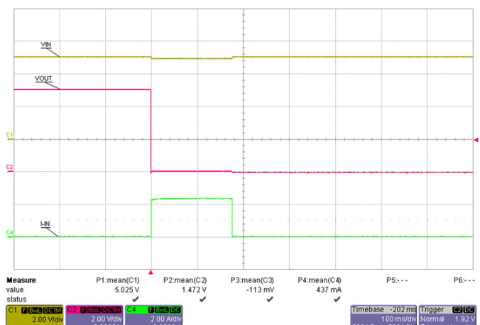
Figure 42. TRANSIENT: THERMAL FAULT LATCHED (TPS2592xL)
