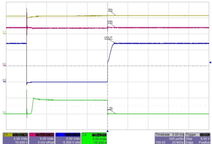
Figure 38. TRANSIENT: RECOVERY FROM SHORT CIRCUIT
