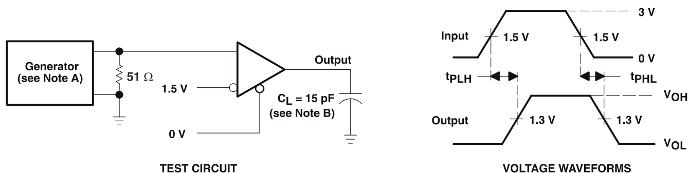
图 6-6. Receiver, V_{OH} and V_{OL}
