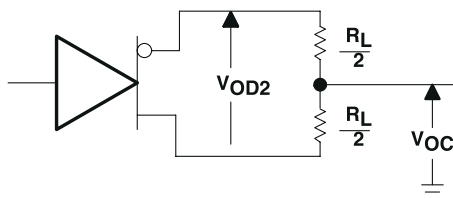
图 6-1. Driver Test Circuit, V_{OD} and V_{OC}
