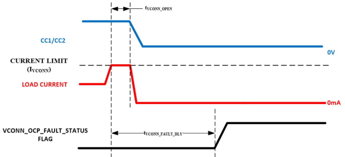
图 2. VCONN Fault Timing
