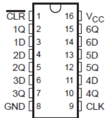
图 5-1. D, DB, DGV, N, NS, or PW Package (Top View)
