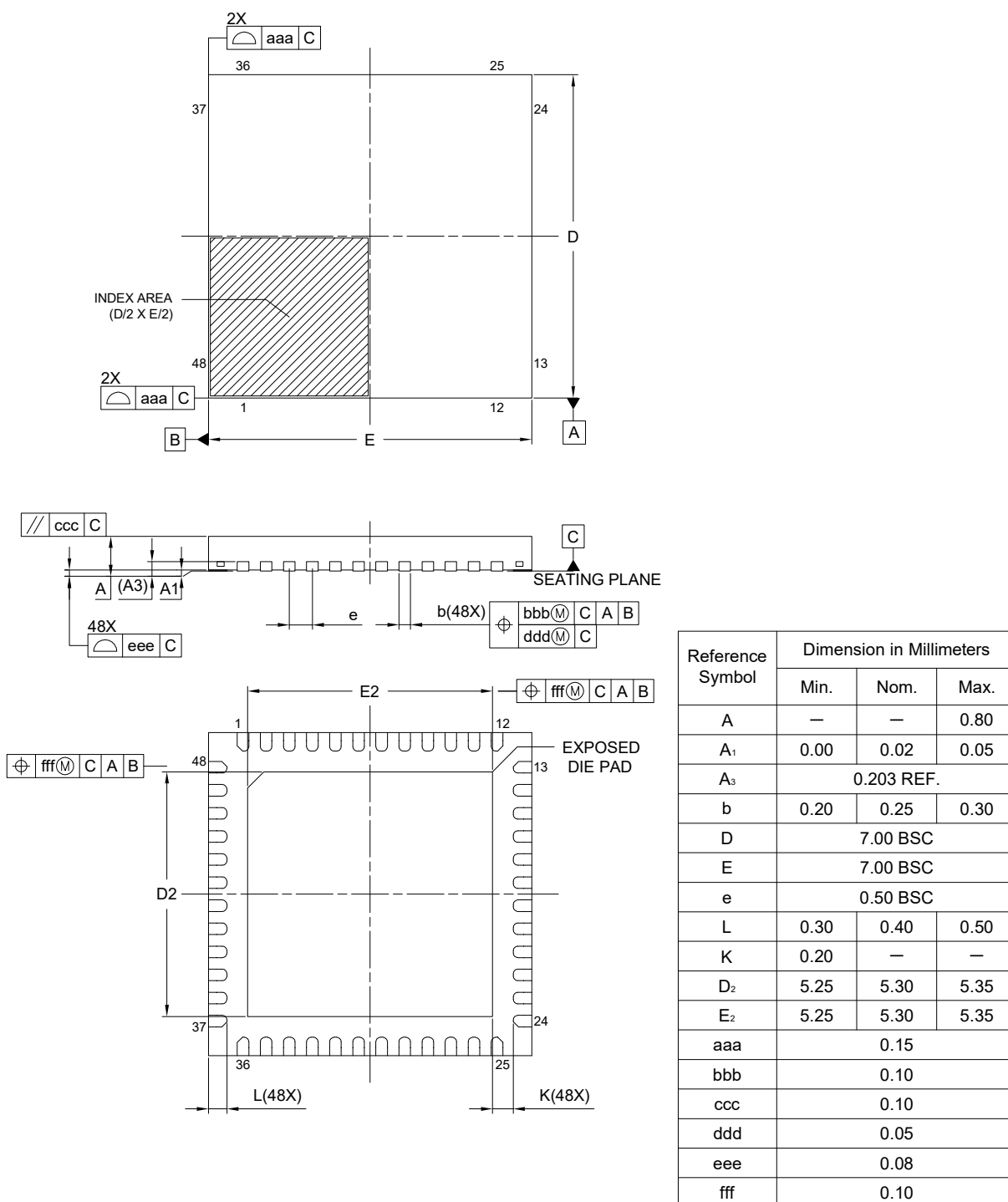
Figure 2.7 HWQFN 48-pin
