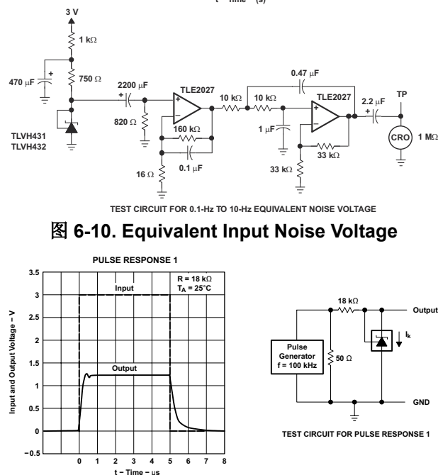
图 6-12. Pulse Response 1
