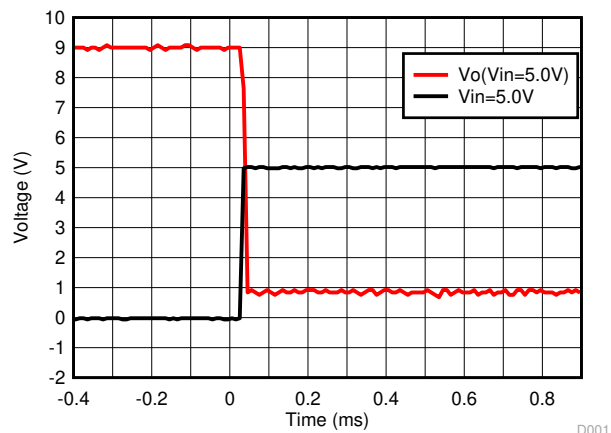
图 9-4. Output Response With Large Overdrive Voltage
