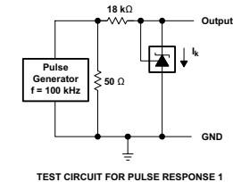
图 6-12. Pulse Response 1
