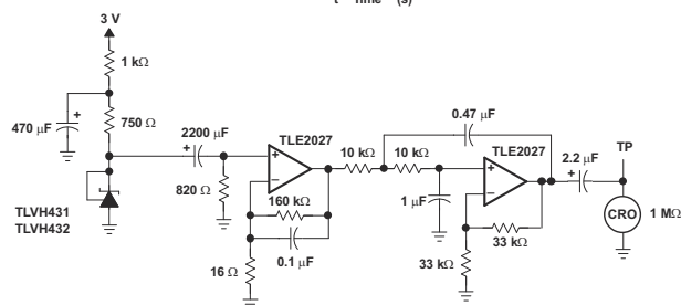
图 6-10. Equivalent Input Noise Voltage
