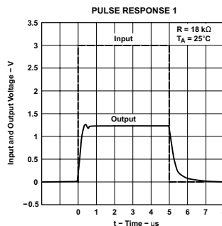
图 6-12. Pulse Response 1
