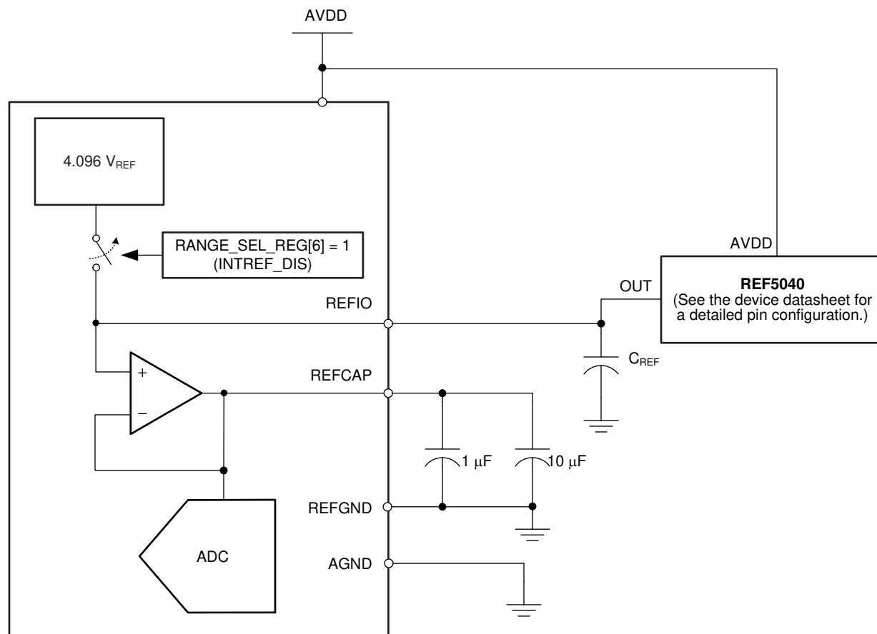
图 7-14. Device Connections for Using an External 4.096-V Reference
