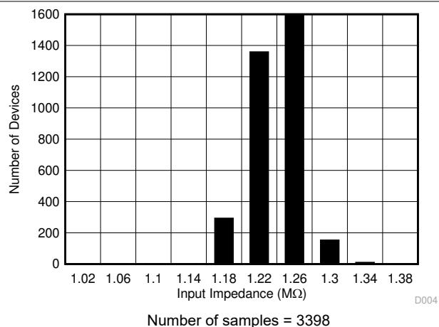
图 6-12. Typical Distribution of Input Impedance
