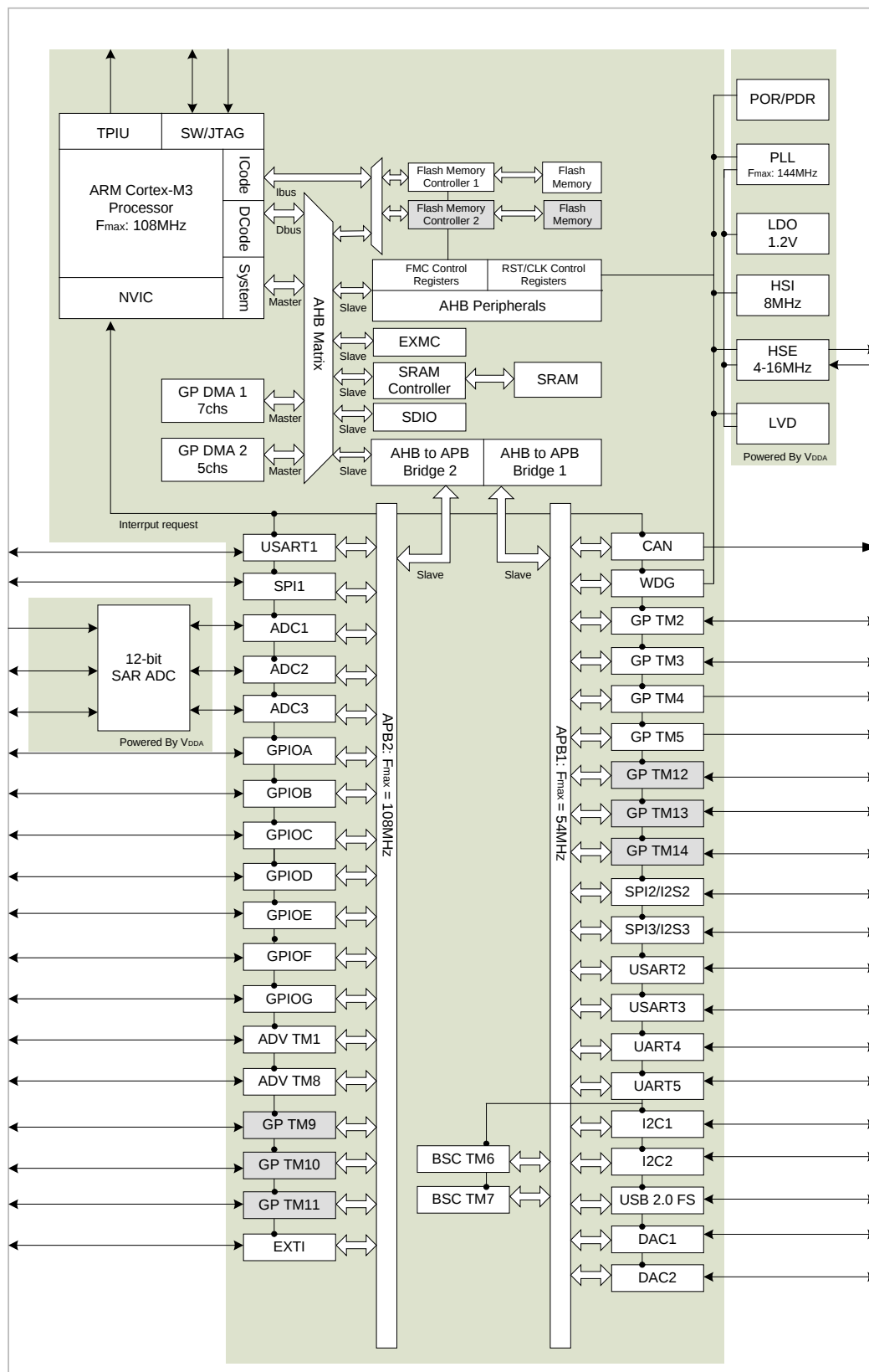
Figure 2. GD32F103xC/D/E/F/G/H/K block diagram
