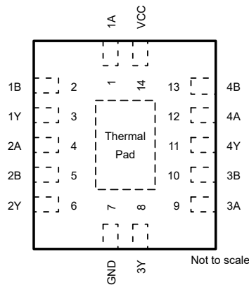
图 5-3. SN74AHC132 BQA Package, 14-Pin WQFN (Top View)
