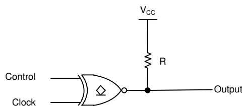
图 9-1. Typical application schematic
