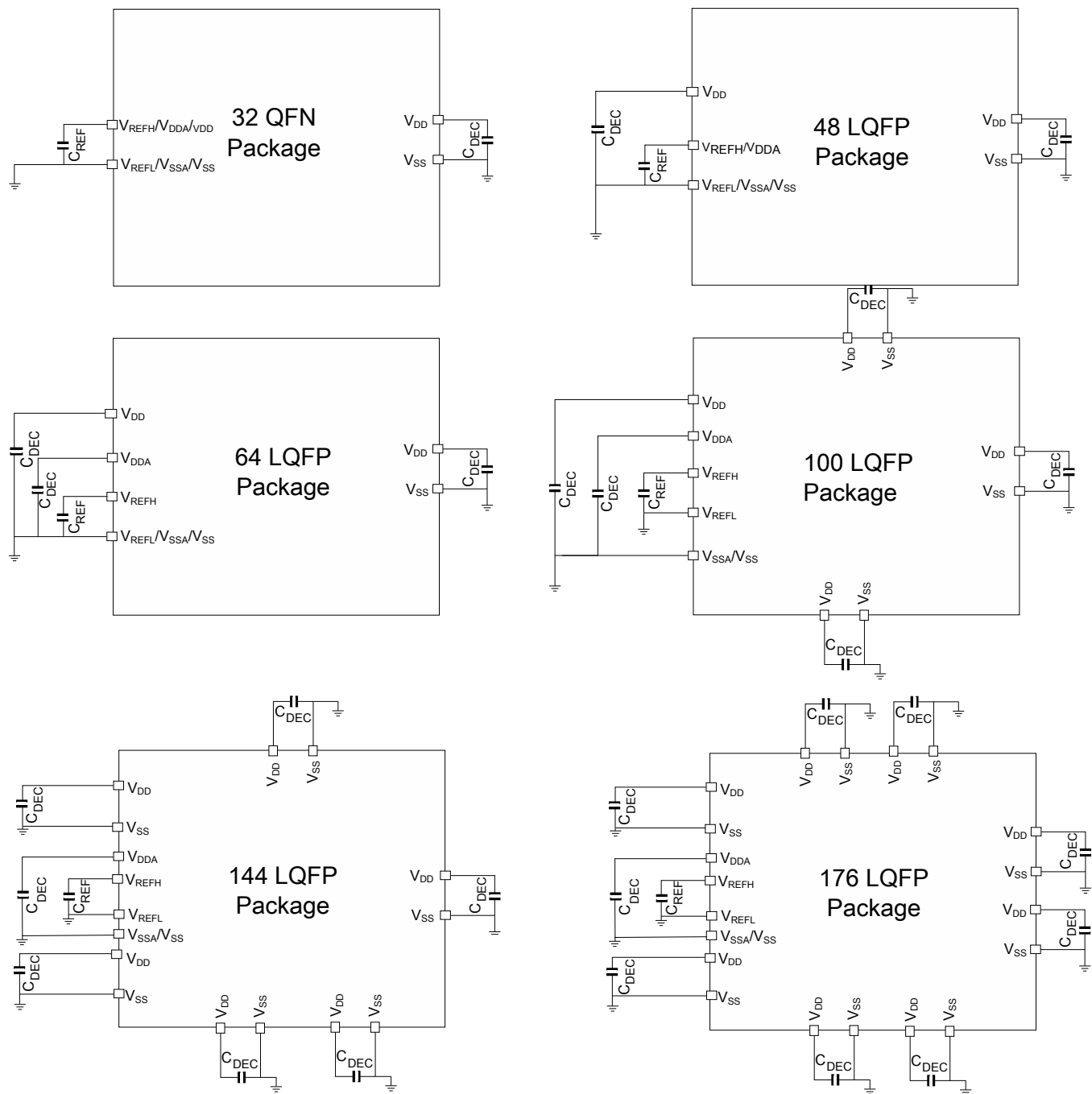
Figure 6. Pinout decoupling
