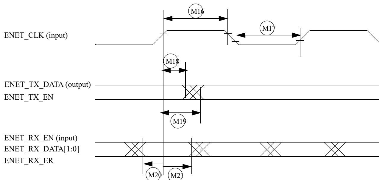
Figure 42. RII mode signal timing diagram
