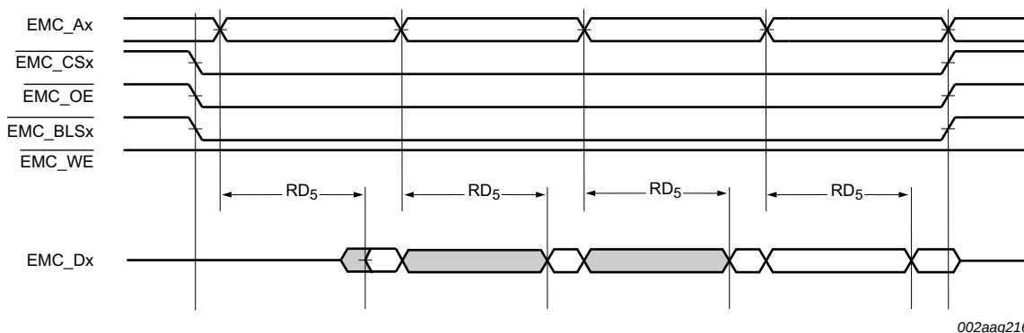
Fig 18. External static memory burst read cycle
