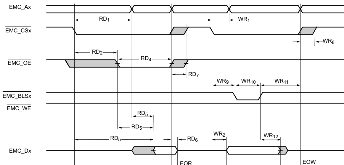
Fig 16. External static memory read/write access ( \text{PB} = 0 )
