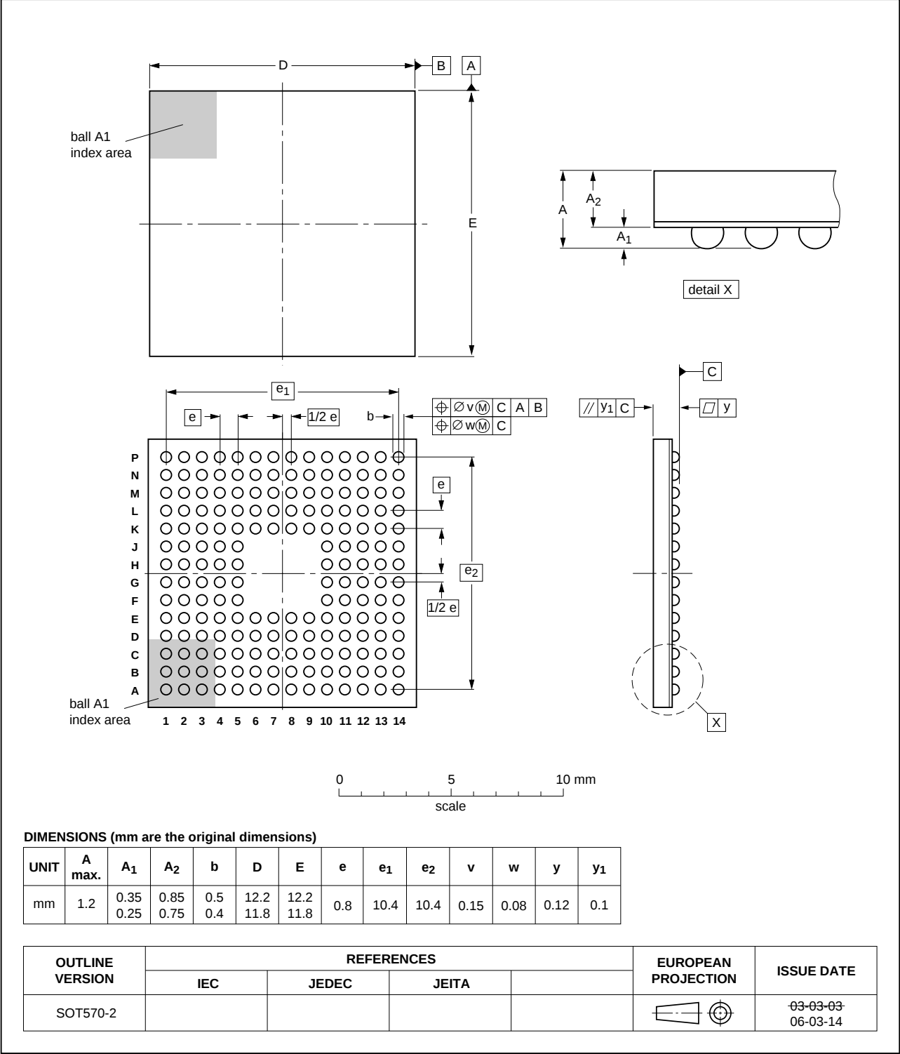
Fig 43. TFBGA180 package
