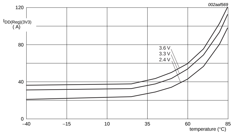
Fig 9. Power-down mode: Typical regulator supply current I_{DD(REG)(3V3)} versus temperature
