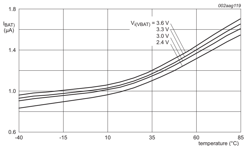
Fig 10. Deep power-down mode: Typical battery supply current I_{BAT} versus temperature
