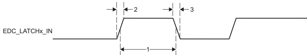
图 7-105. PRU-ICSS ECAT LATCHx_IN Timing
