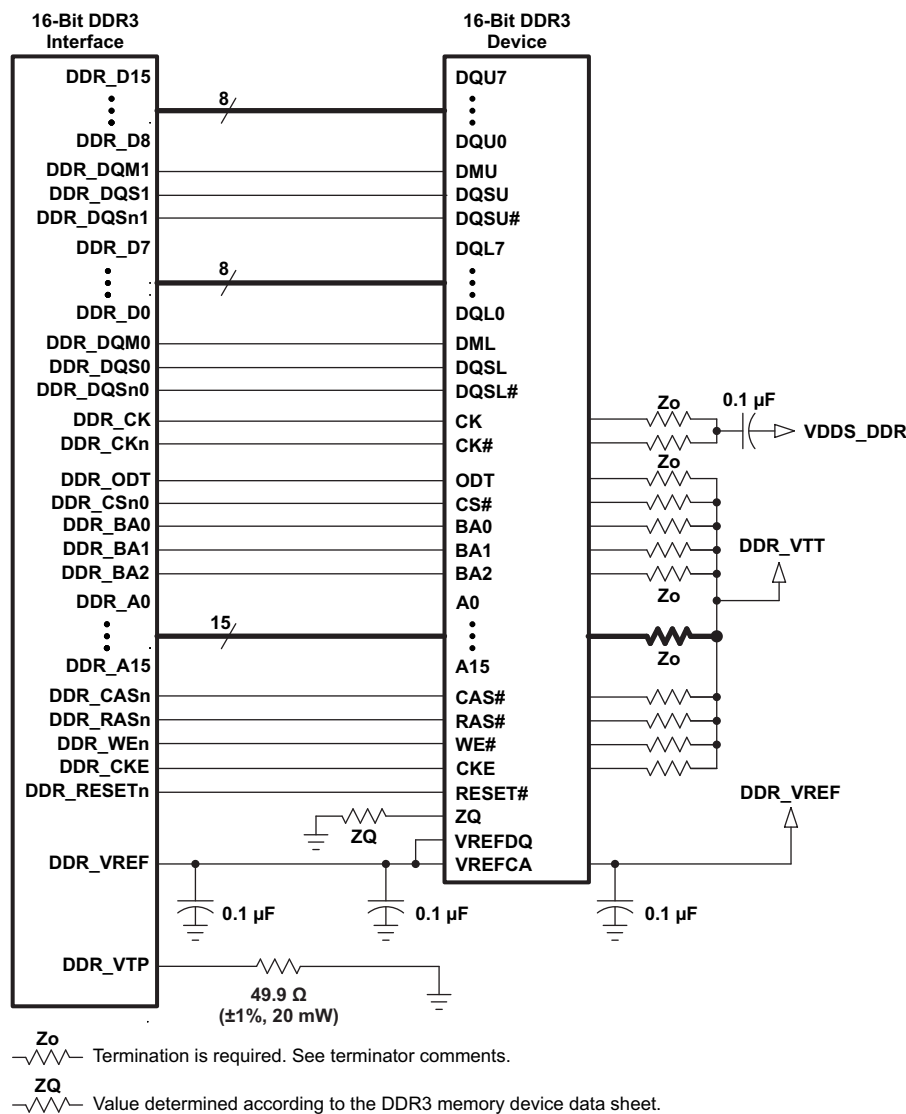
Figure 7-47. 16-Bit DDR3 Interface Using One 16-Bit DDR3 Device with V_{\Pi} Termination
