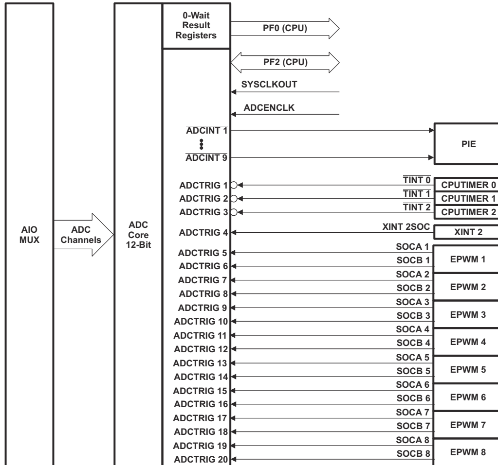
图 8-21. ADC Connections
